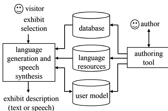
Figure 1: M-PIRO's system architecture
