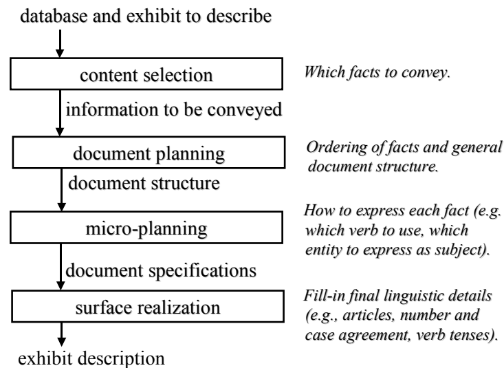
Figure 6: Stages of natural language generation in M-PIRO
