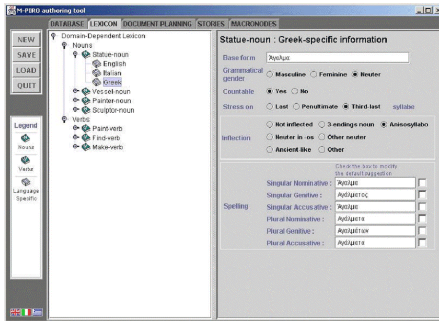
Figure 7: Updating the domain-dependent lexicon
