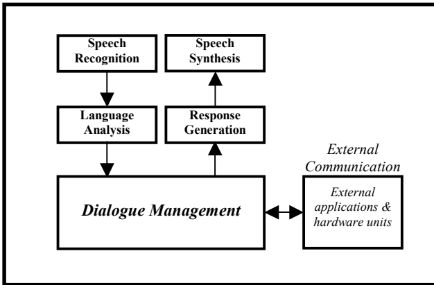
Figure 1: Architecture of spoken dialogue systems
